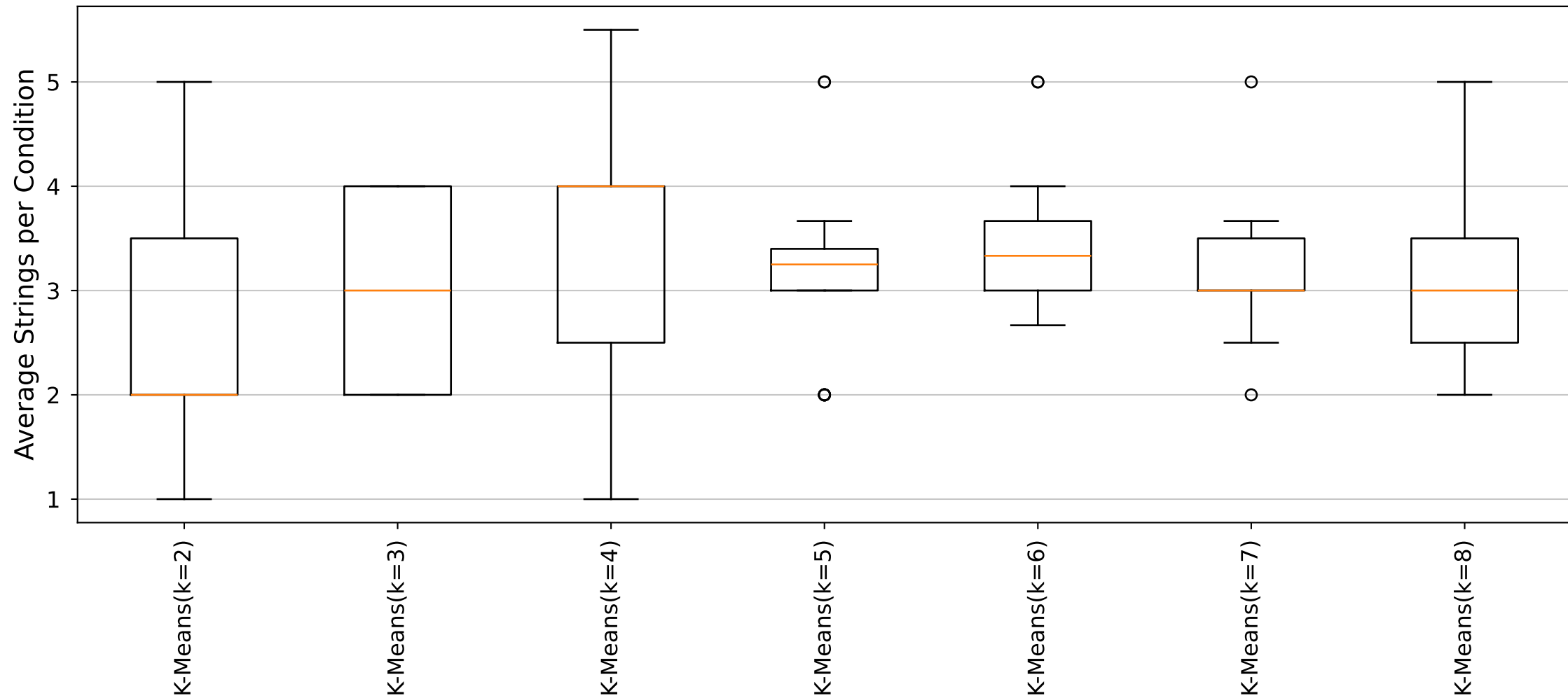
YARA Rules Average Strings per Condition Distribution (Cluster16_Size8 dataset)
